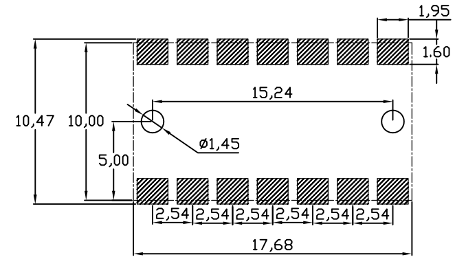
RECOMMENDED PCB LAYOUT TOP VIEW (.XX±0.05)
